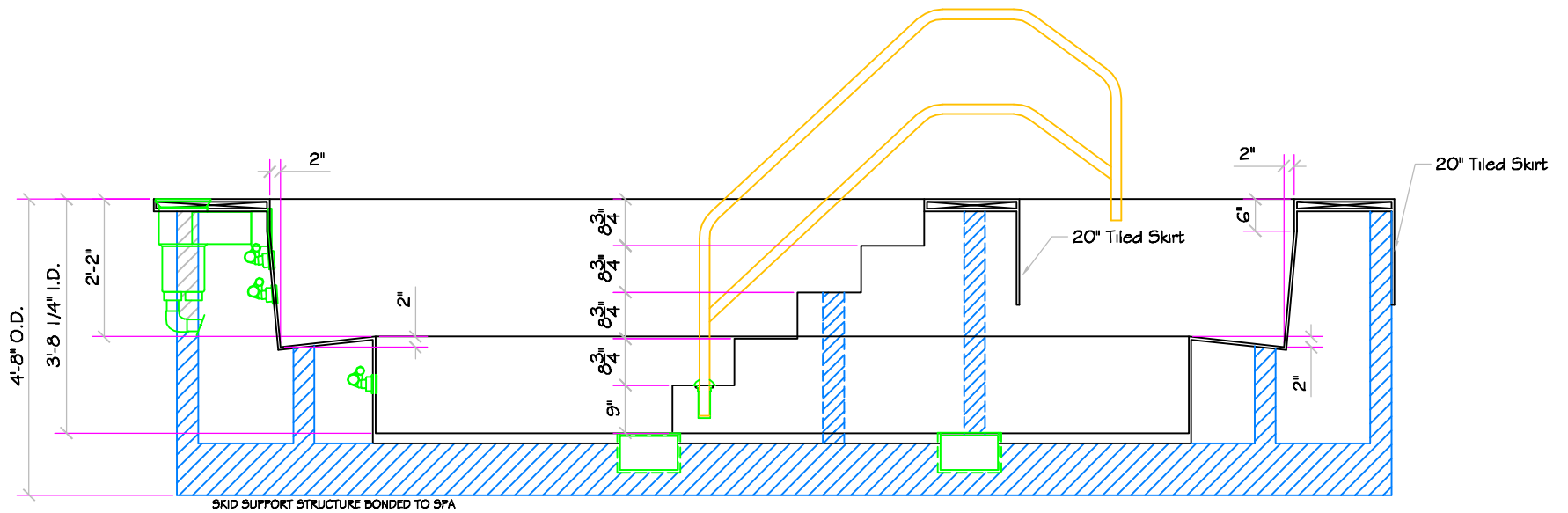
SECTION A
