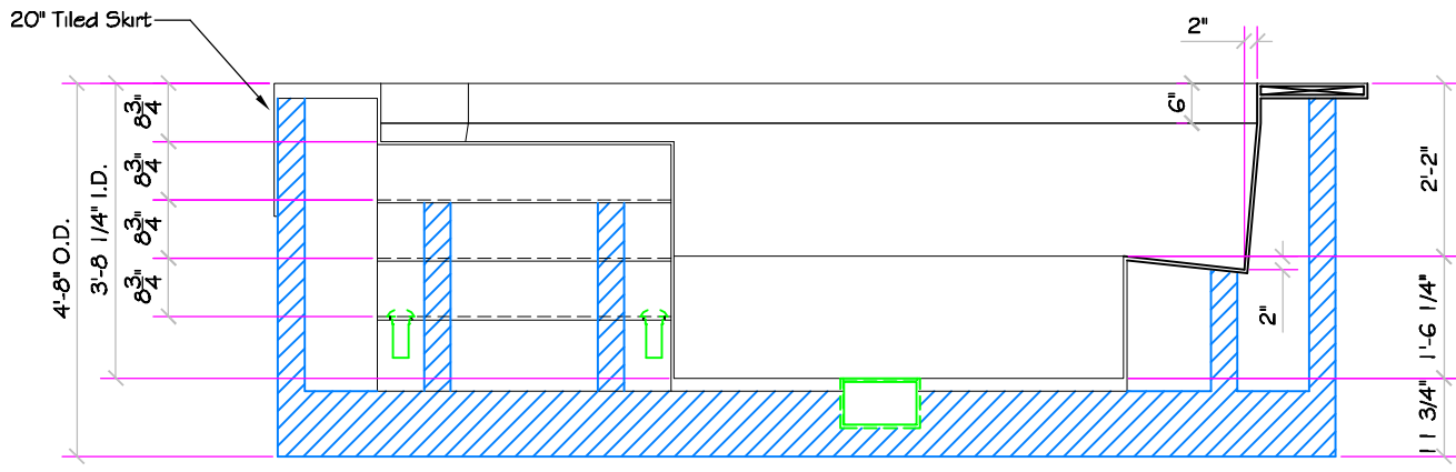
SECTION B
