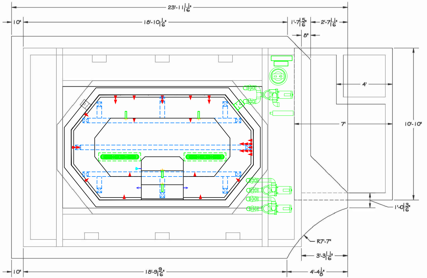
PLAN SCALE 1/2" = 1'
