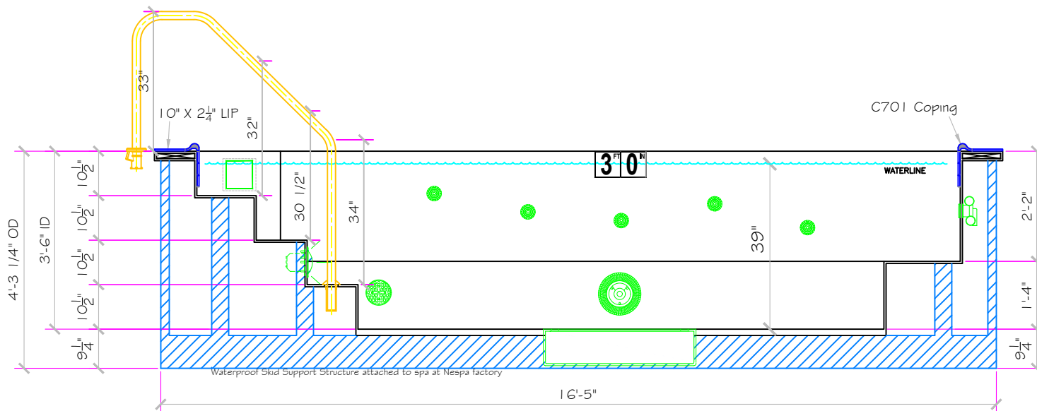
Interior Section
