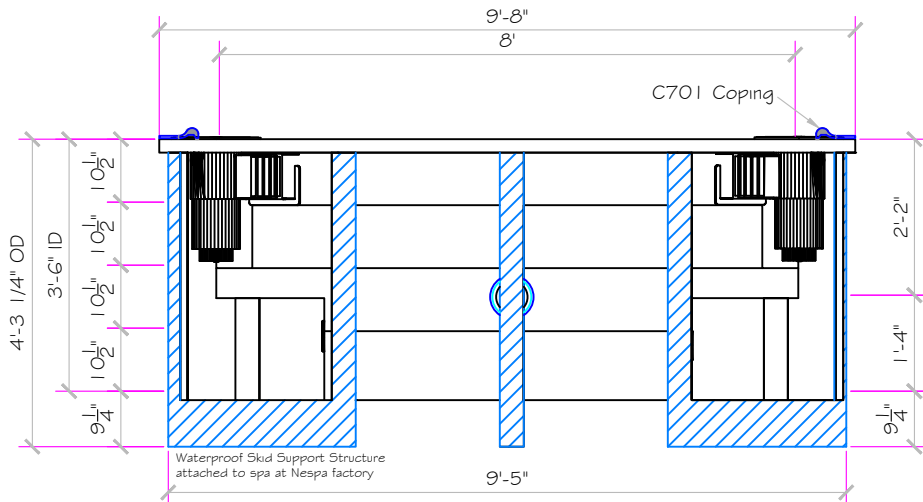
Exterior Elevation
