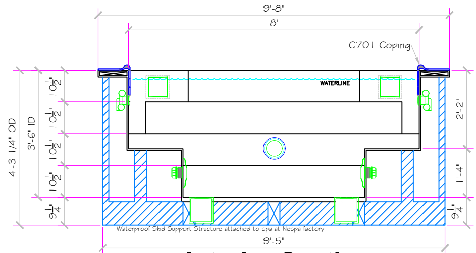
Interior Section
